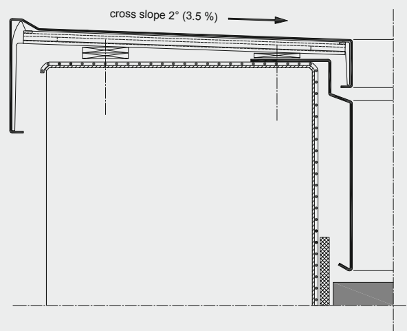
Wall capping profile MAG-6 with additional fascia board (bent)
