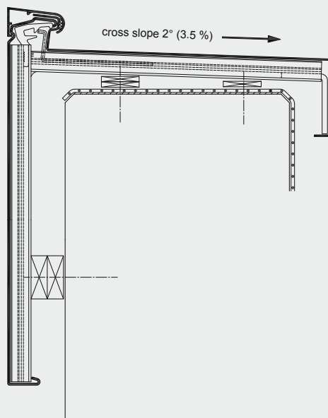
Wall capping profile TAG-MA (TA-MA)
