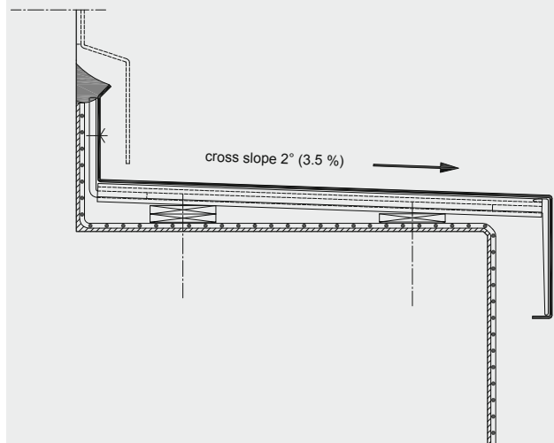
Window sill capping (bent) or cornice capping (bent)
