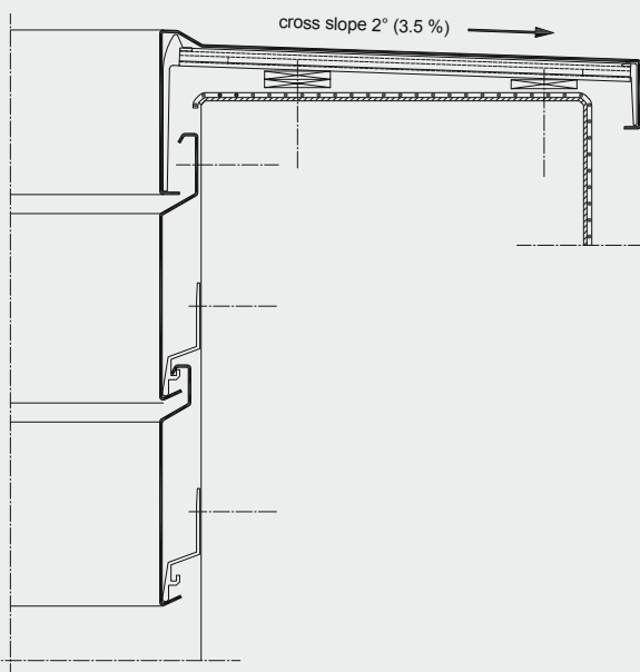
Wall capping profile MAG-6 with additional fascia board ZBK
