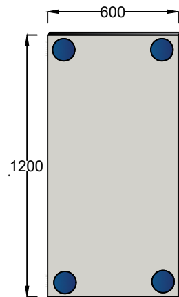
600mmx1200mm boards Minimum 4.No. Fixings
