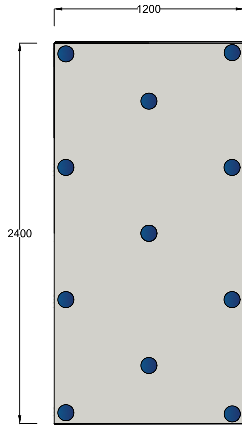
Main Roof Zone Minimum 11.No. Fixings
