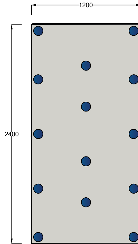
Perimeter Zone Minimum 14.No. Fixings
