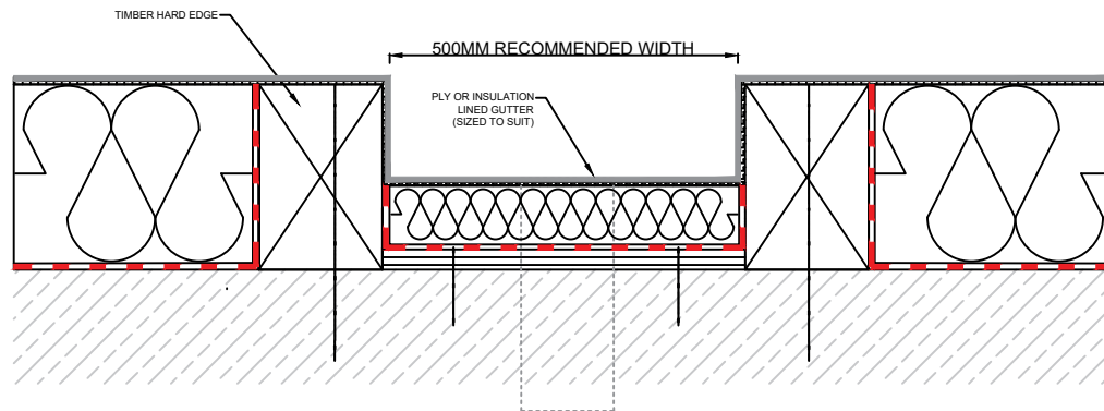
CENTRAL GUTTER
