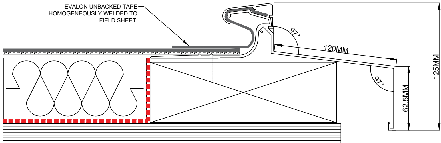
BRACKET RECESS DETAIL
