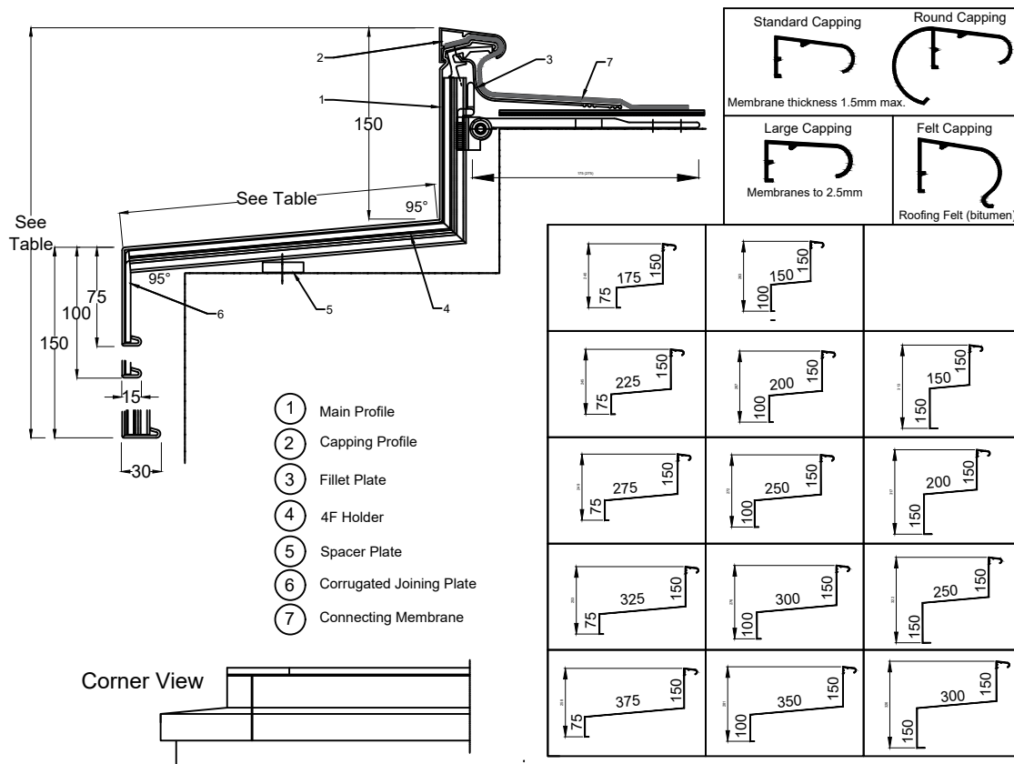
Art Line 1 - Standard Profile Sizes
