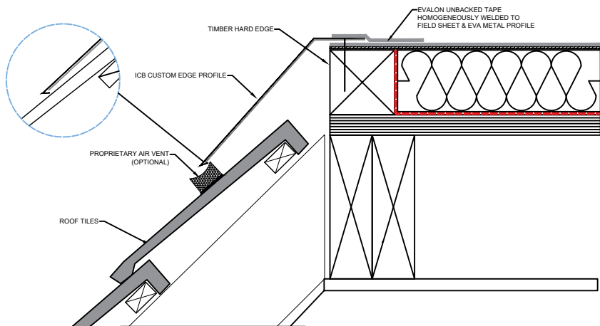
WARM ROOF
