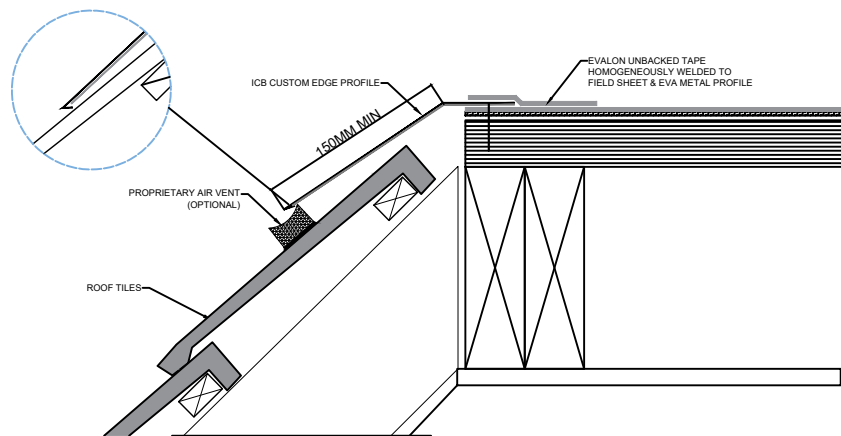
COLD ROOF
