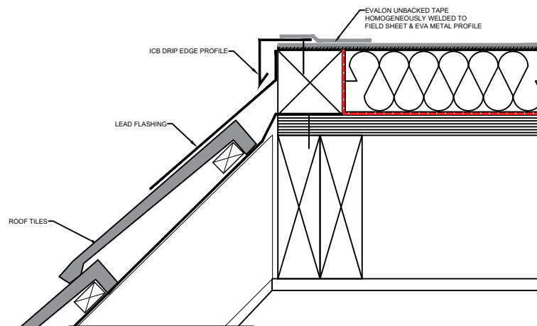
WARM ROOF
